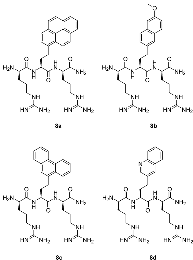
Figure 1. Tripeptides generated from the building blocks 8a–d by standard Fmoc solid-phase synthesis. [15] The non-protonated form is shown.
