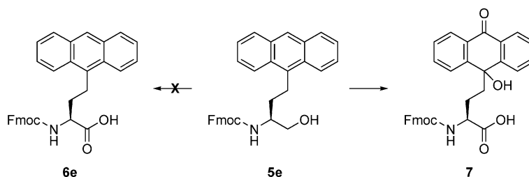
Scheme 2. Oxidation of the anthracene amino alcohol 5e with PDC in \text{DMF} .
