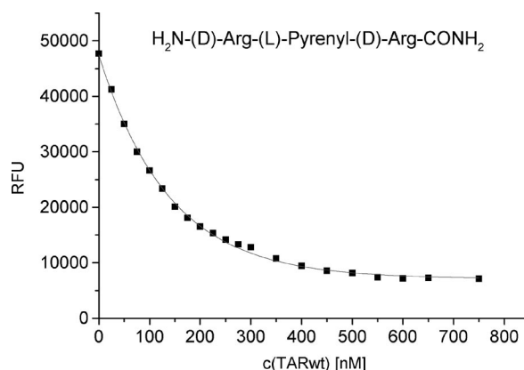
Figure 3. Fluorescence titration of peptide 8a with TAR 10 . Assay conditions: 100 nM pyrene peptide 8a , 50 mM Tris-HCl, pH = 7.4, 20 mM KCl, 0.01% Triton-X100; \lambda_{ex} = 340 nm, \lambda_{em} = 400 nm. The solid line shows the best fit of a 1:1 binding model to the experimental data points.
