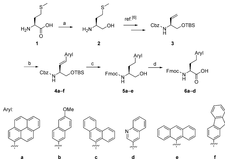
Scheme 1. Reagents: (a) \text{LiBH}_4 , \text{TMSCl} , \text{THF} ; (b) aryl-Br, \text{Pd}(\text{OAc})_2 , \text{K}_2\text{CO}_3 , \text{Bu}_4\text{NOTf} , \text{DMF}/\text{H}_2\text{O} ; (c) (1) 1,4-cyclohexadiene, \text{Pd}(\text{OH})_2 or \text{H}_2 , \text{Pd}/\text{C} for 4b , (2) TBAF, (3) Fmoc-OSu; (d) PDC, \text{DMF} .
