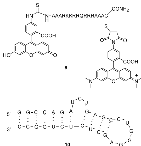
Figure 2. Structures of the Tat peptide 9 and the HIV-1 TAR RNA model 10 .
